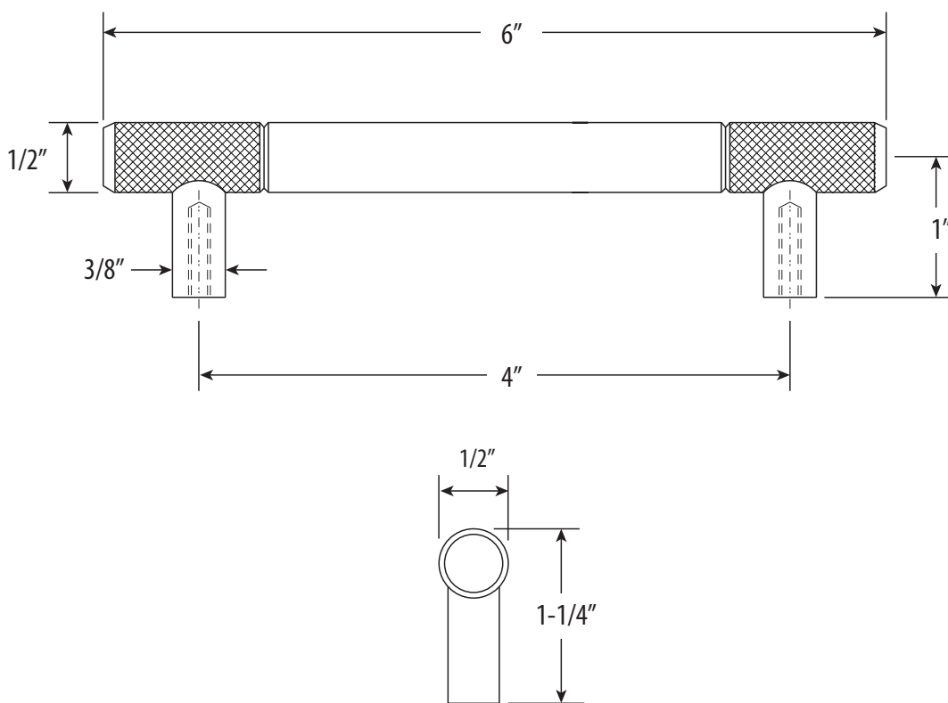
END VIEW
