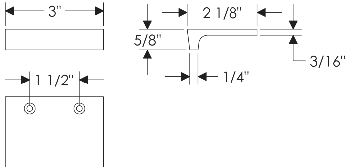
CK213 Catch Pull 3"
