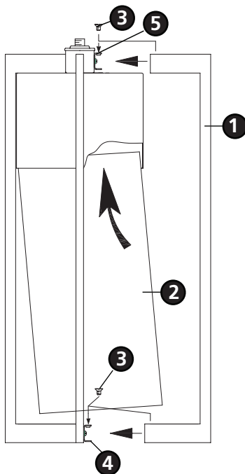
Drawing 3 - Glass Installation
